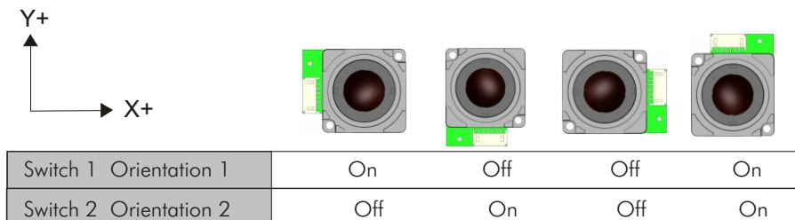
Figure.1 Mounting Orientations
